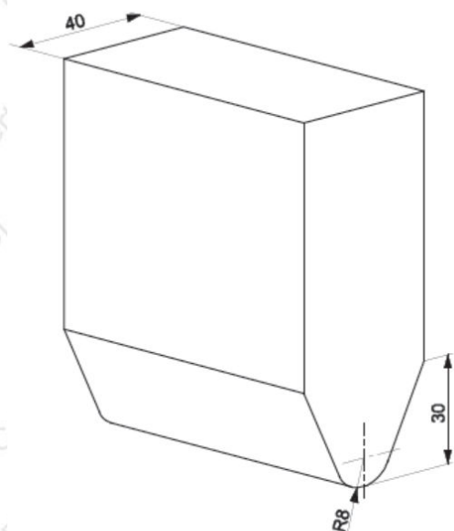
Figure 39 — Striker dimensions
